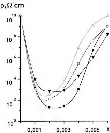
Fig. 3. Resistivity of the \text{Ba}(\text{Ti}_{1-x}\text{M}_x)\text{O}_3 ceramic as a function of the degree of aliovalent substitution: \text{M}=\text{Nb} (■); \text{Ta} (□); \text{Mo} (▼); \text{W} (△); T=20^\circ\text{C} .
