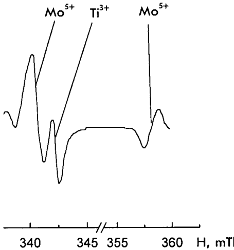
Fig. 4. EPR spectra of the \text{Ba}(\text{Ti}_{0.999}\text{Mo}_{0.001})\text{O}_3 ceramic; T=20^\circ\text{C} .
