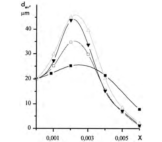
Fig. 2. Average grain size of the \text{Ba}(\text{Ti}_{1-x}\text{M}_x)\text{O}_3 ceramic as a function of the degree of aliovalent substitution: \text{M}=\text{Nb} (■); \text{Ta} (□); \text{Mo} (▼); \text{W} (△).
