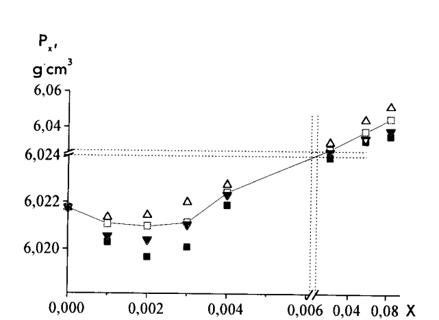
Fig. 1. X-ray density ( P_x ) of the \text{Ba}(\text{Ti}_{1-x}\text{M}_x)\text{O}_3 ceramic as a function of the degree of aliovalent substitution: \text{M}=\text{Nb} (■); \text{Ta} (□); \text{Mo} (▼); \text{W} (△).
